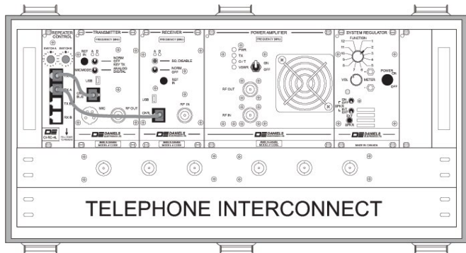
TOP VIEW OF TRANSPORTABLE CASE WITH LID REMOVED
